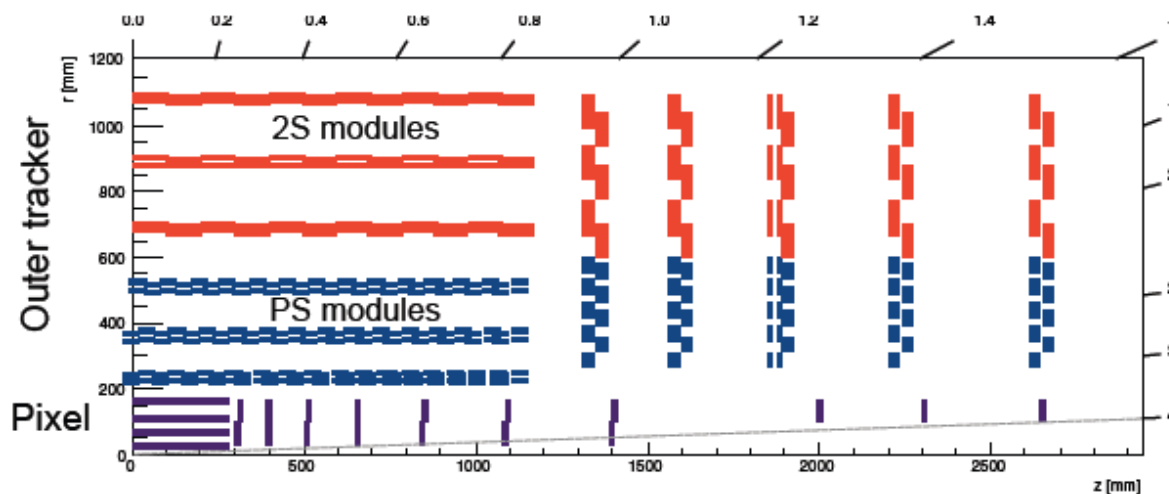
Baseline layout of CMS tracker
