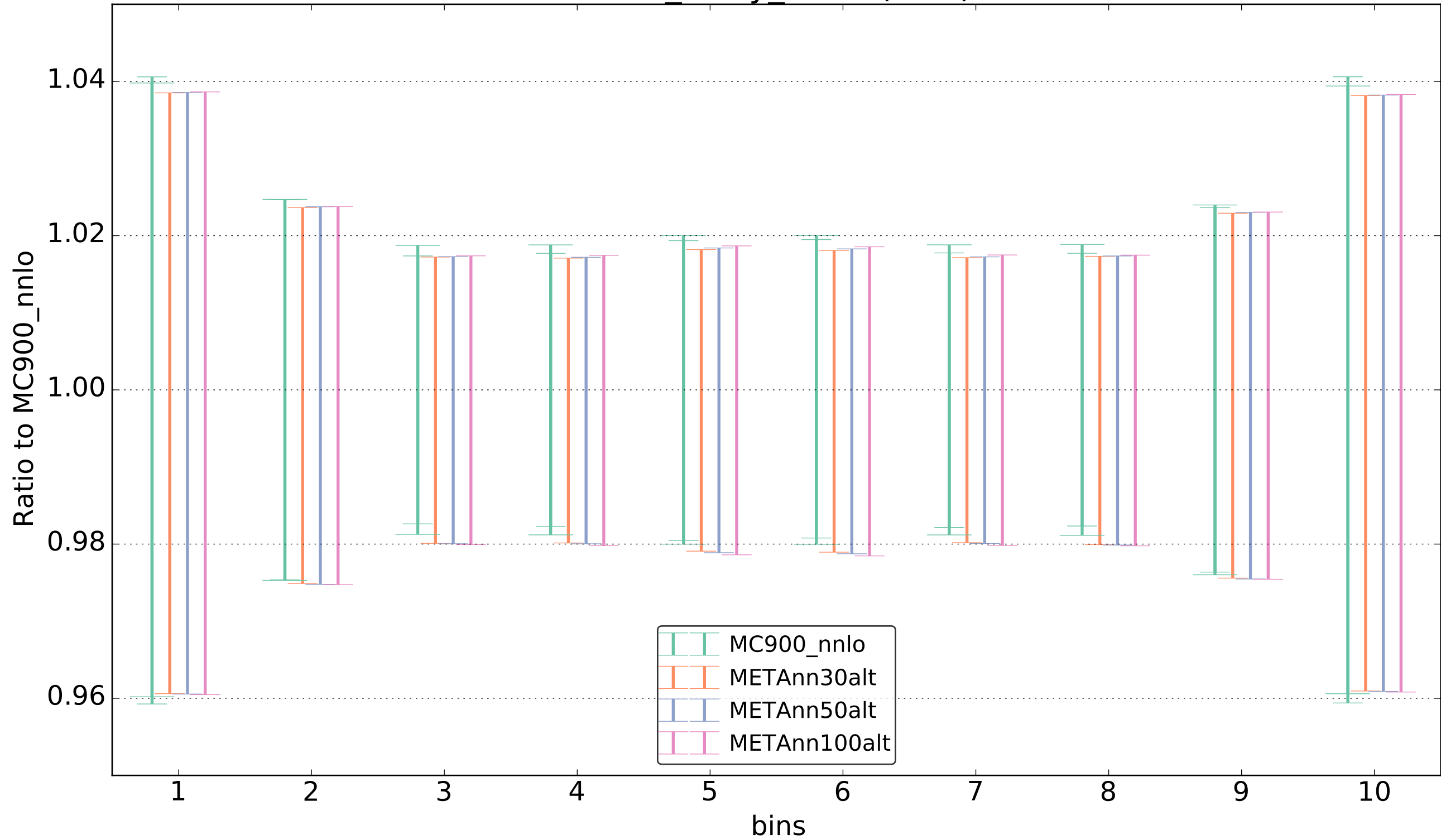
ttbar tbary_13tev(NLO)
